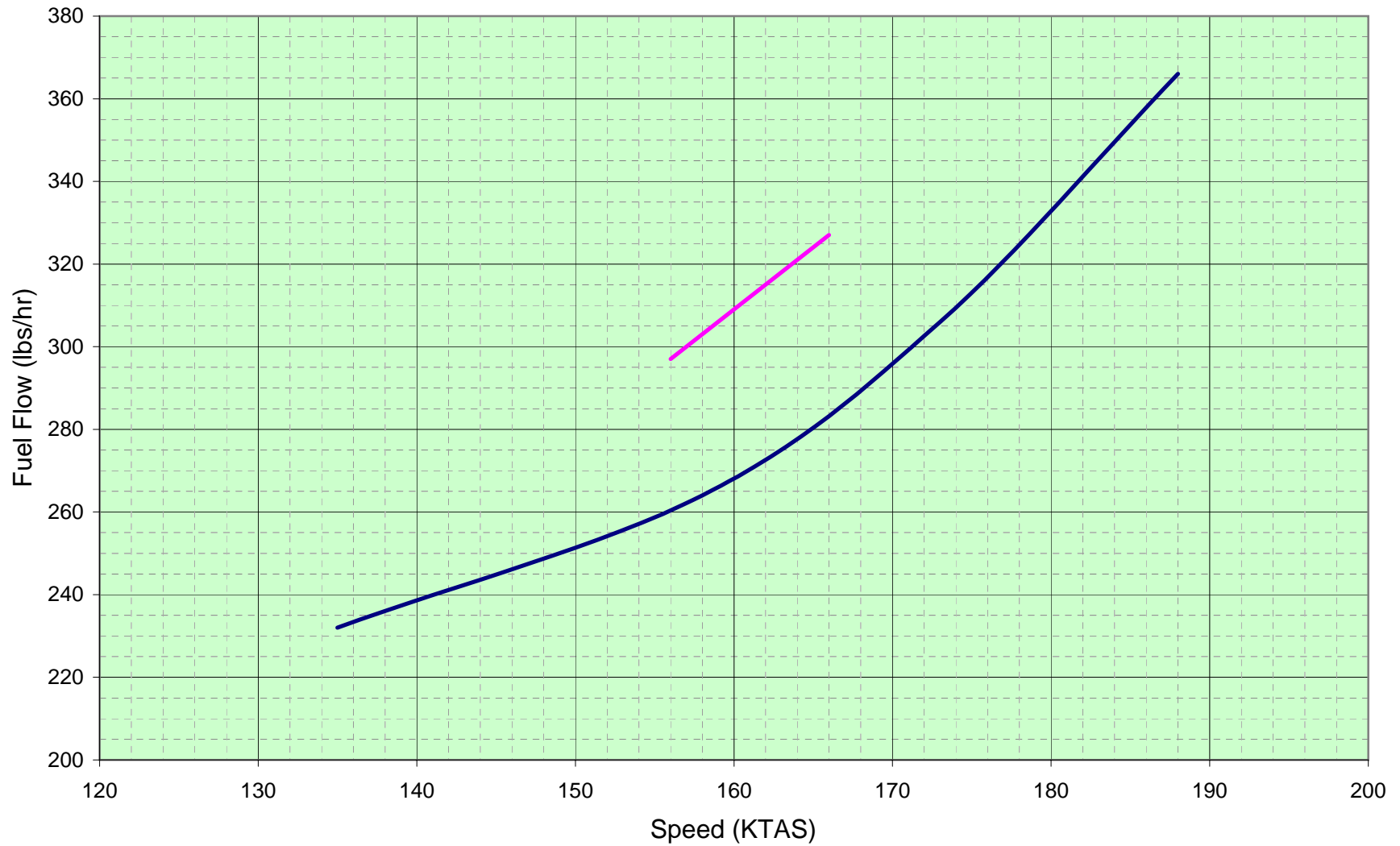
Fuel Flow vs. Speed (13K @ -5C and 96% rpm)
